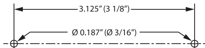
Mounting Template
