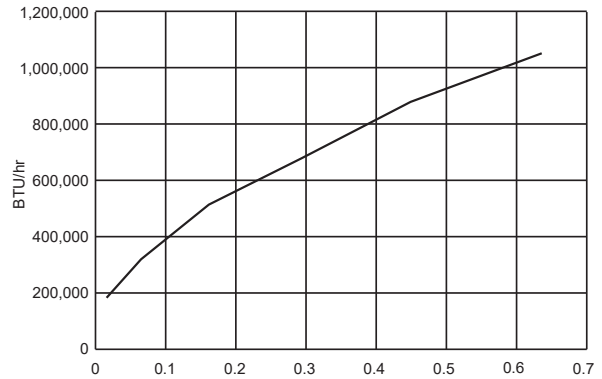
Chart 1 - BTU/hr vs. Differential Pressure (Inches W.C.)
