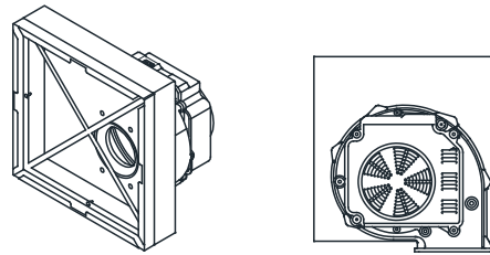
Figure 1 - Filter Box
