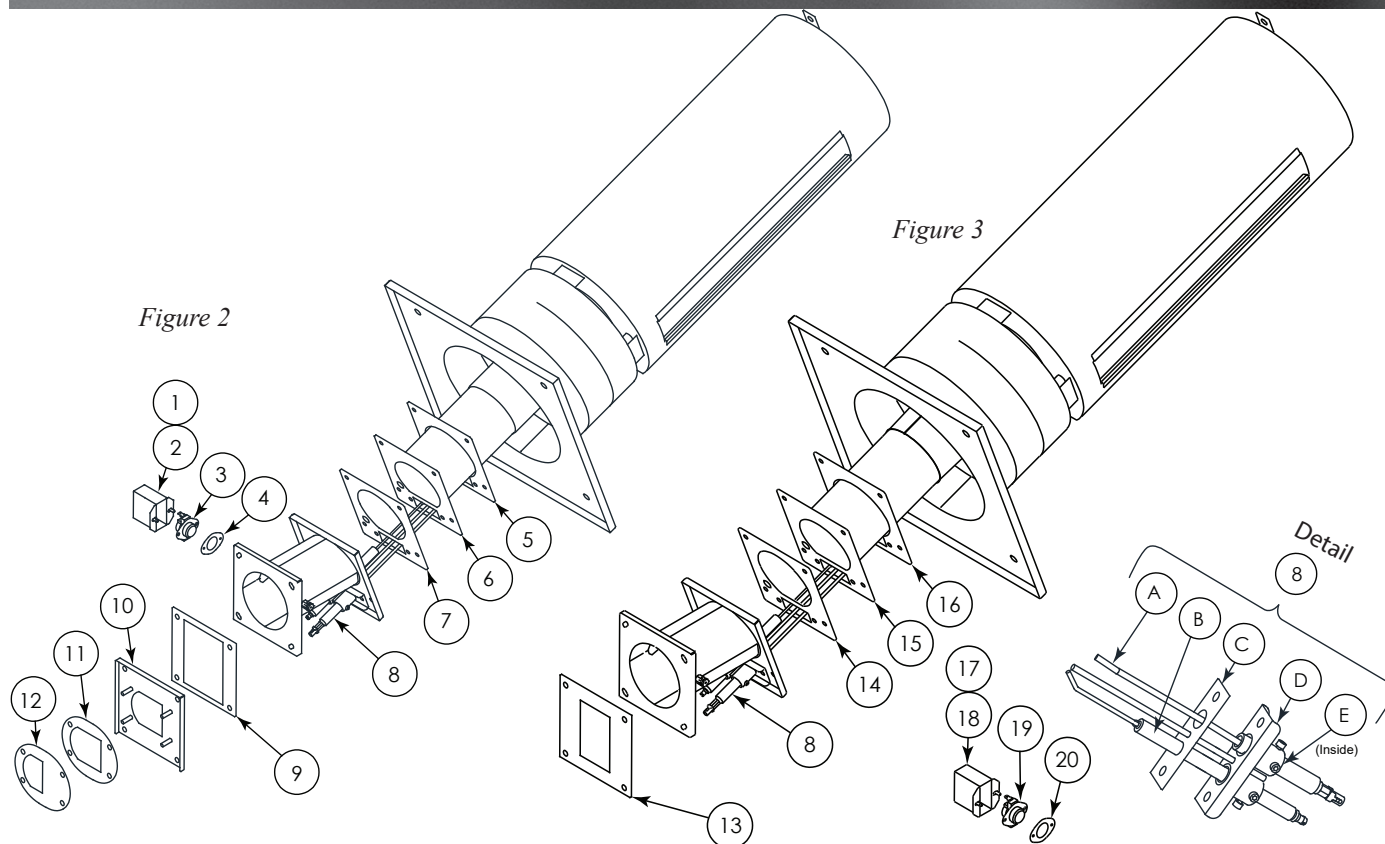
Figure 2 - LNB 500 6" Insertion Combustion Chamber Expanded View
